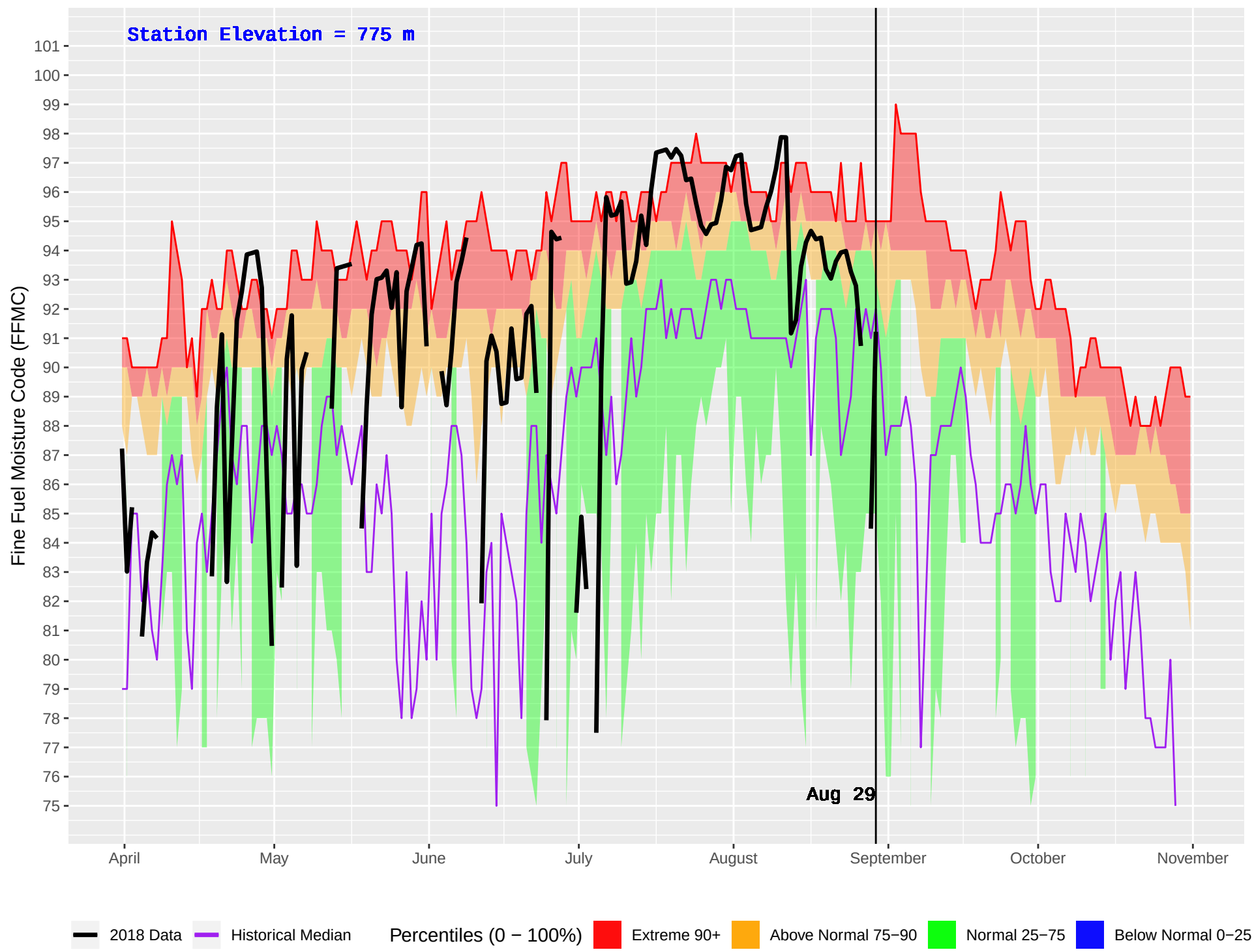
ELKO (412) : Historical (1970–2016) and Current (2018) Daily Fine Fuel Moisture Code (FFMC)
