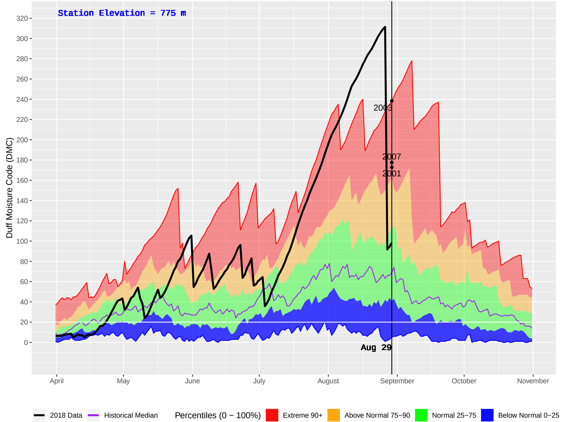
ELKO (412) : Historical (1970–2016) and Current (2018) Daily Duff Moisture Code (DMC)
