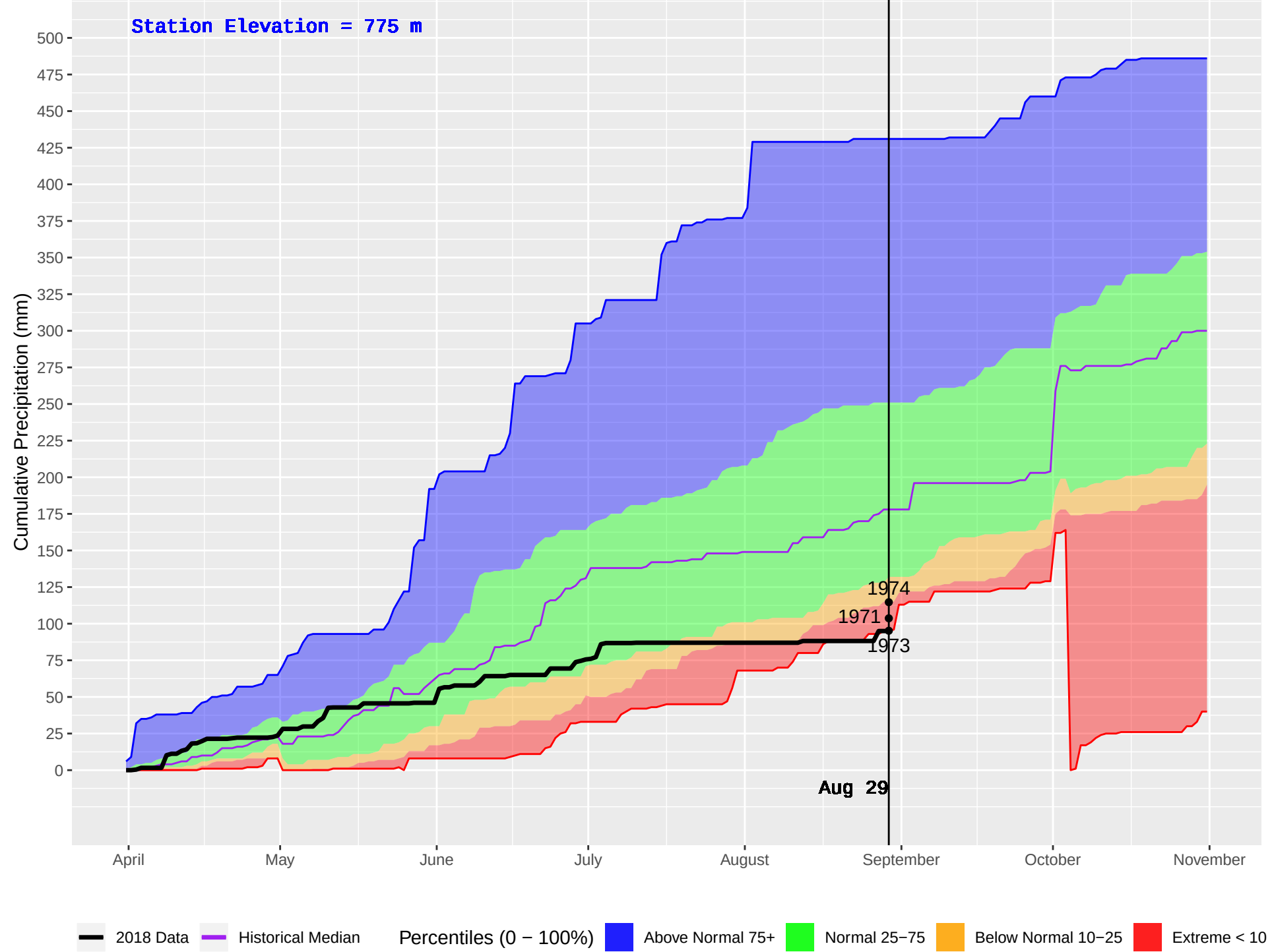
ELKO (412) : Historical (1970–2016) and Current (2018) Daily Cumulative Precipitation
