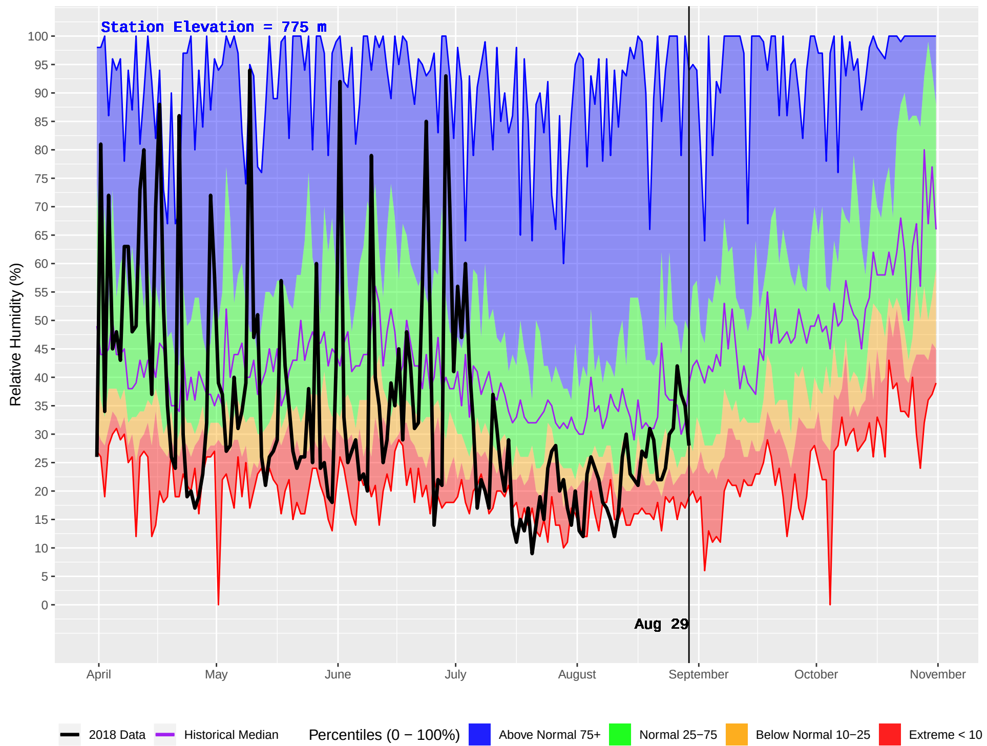
ELKO (412) : Historical (1970–2016) and Current (2018) Daily Relative Humidity
