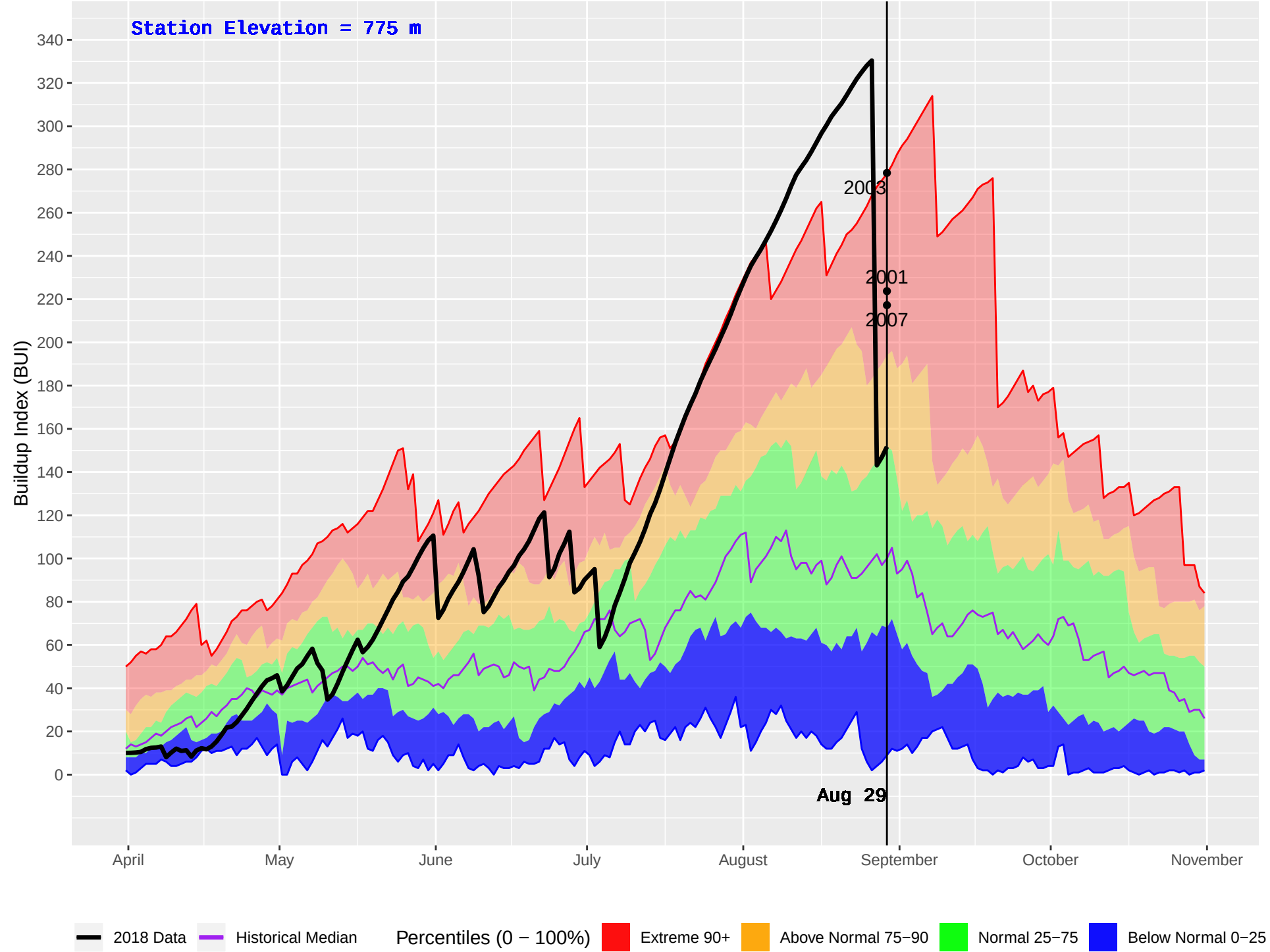
ELKO (412) : Historical (1970–2016) and Current (2018) Daily Buildup Index (BUI)
