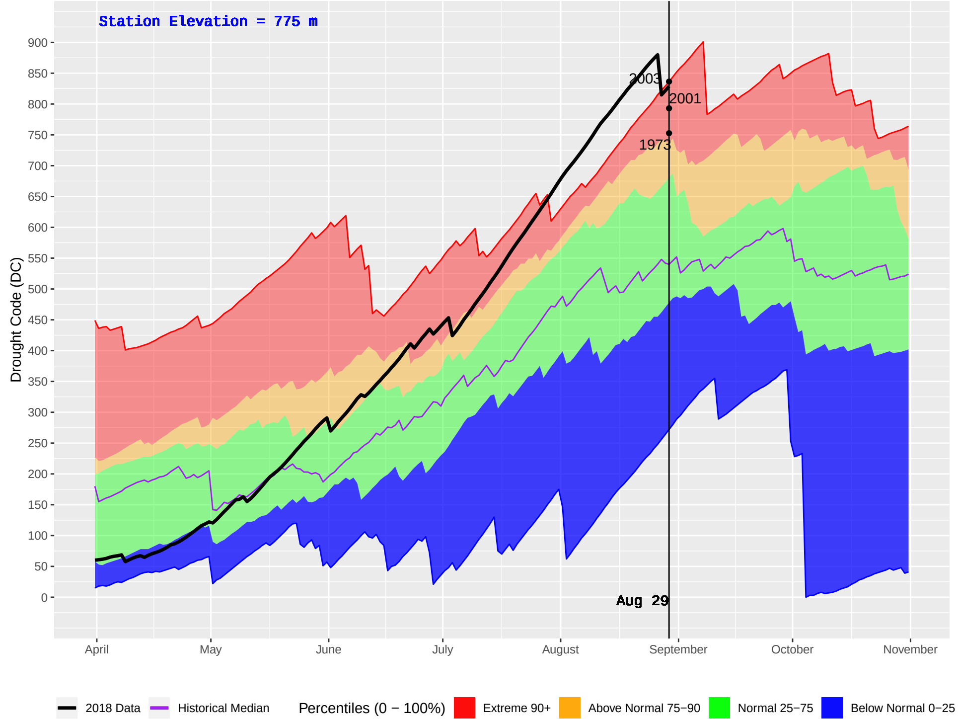
ELKO (412) : Historical (1970–2016) and Current (2018) Daily Drought Code (DC)
