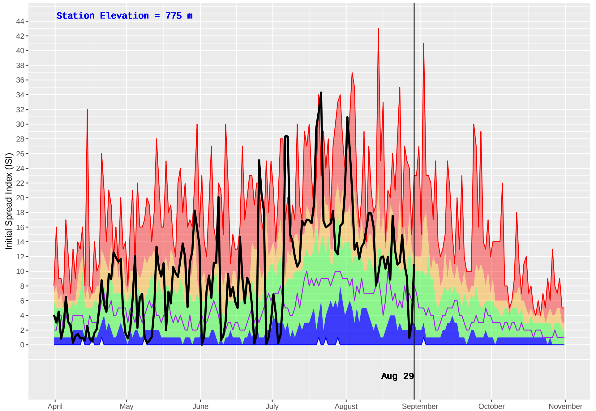
ELKO (412) : Historical (1970–2016) and Current (2018) Daily Initial Spread Index (ISI)
