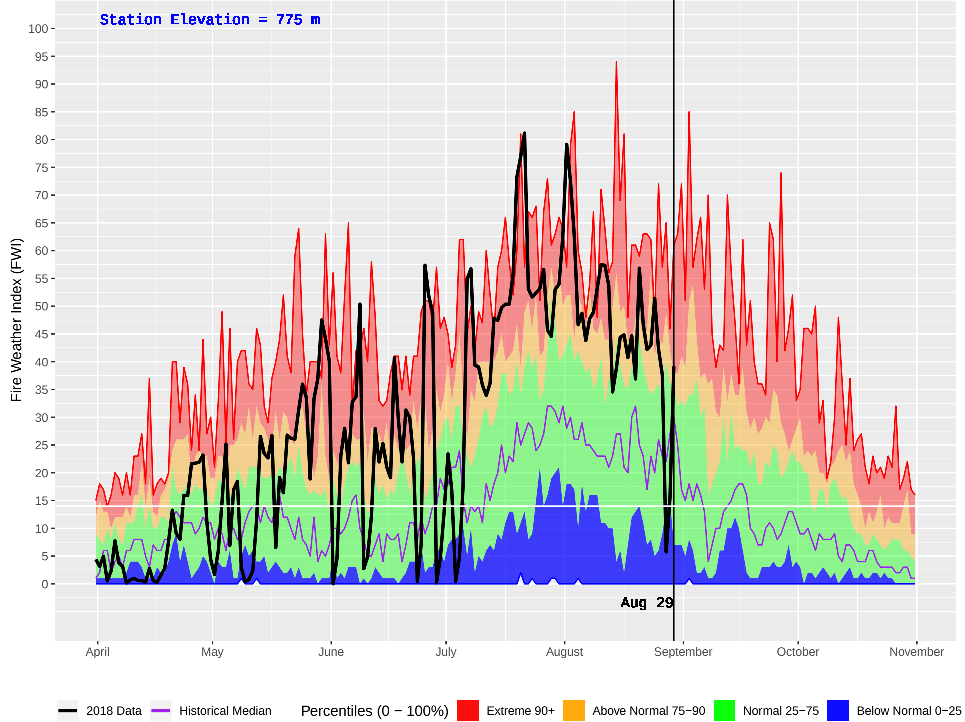
ELKO (412) : Historical (1970–2016) and Current (2018) Daily Fire Weather Index (FWI)
